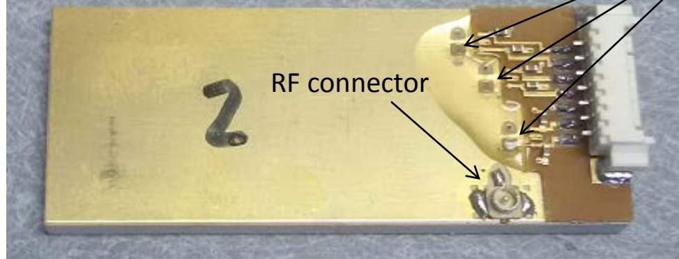
Bottom View (Ground plane side /switching circuitry)
