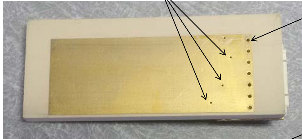
Top View (Patch radiator side)
